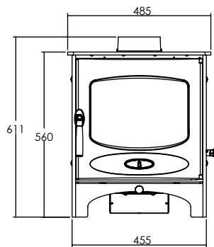
Standard Model
