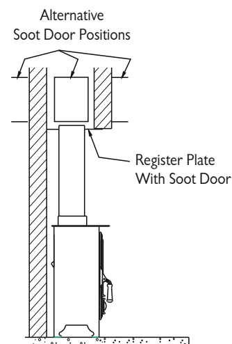
Fig. 6 Horizontal Register Plate With Top Flue Connection
