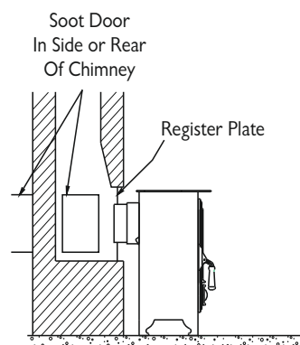
Fig. 4. Vertical Register Plate With Bricked Up Fireplace
