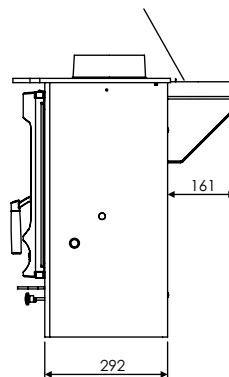
Optional Vertical Rear Flue Adapter
