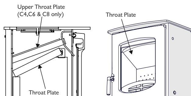
Fig.3. Throat Plate Position and Lowering
