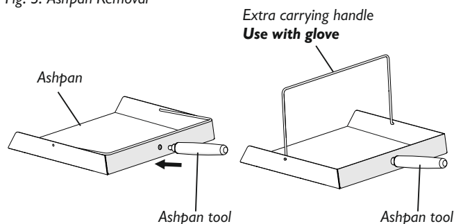
Fig. 3. Ashpan Removal
