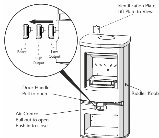
Fig. 3 Stove controls
